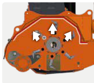
Controtelaio interno "Full Coverage" in Strenx 700. Double skin mulching frame with interanl "Full Coverage" layer in Strenx 700.
